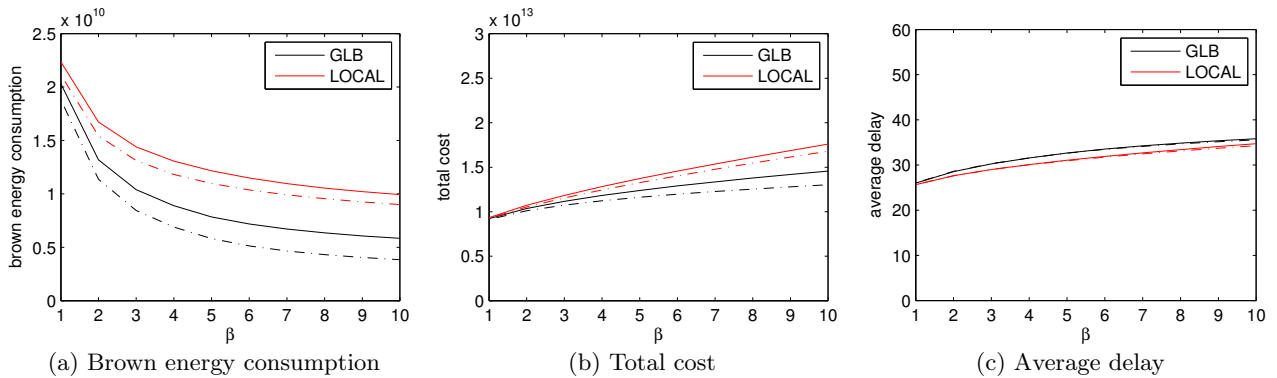
Figure 4: Comparison of GLB and LOCAL as a function of \beta . The renewable capacity is 2. The dashed line is the same setting except with storage.
