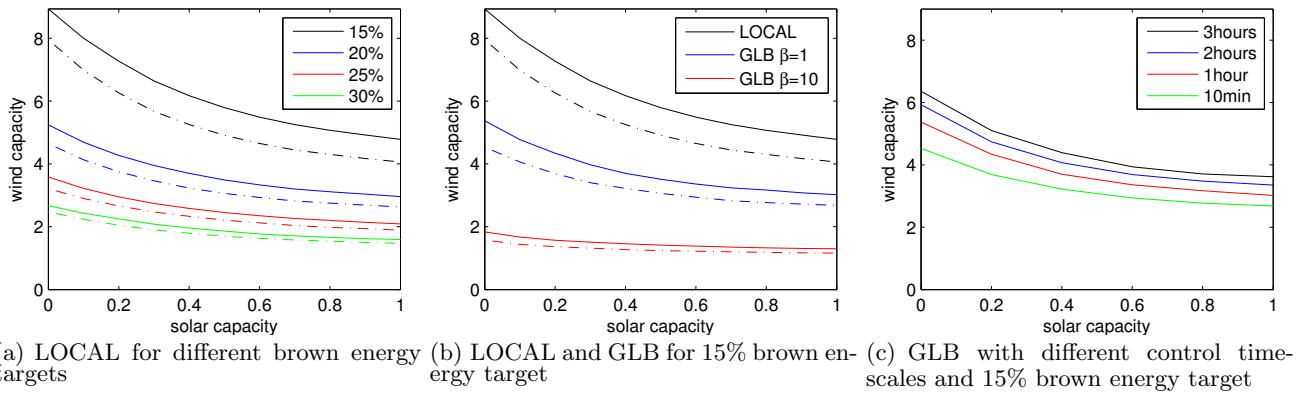
Figure 6: Wind and solar capacity required to reduce brown energy usage to 15–30% of the baseline, as a function of solar capacity. The dashed line is the same setting except with storage.
