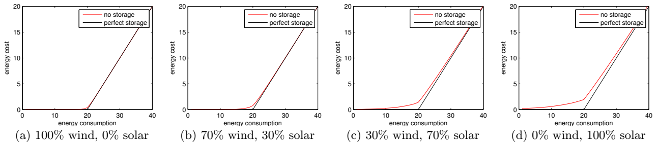
Figure 3: Energy cost as a function of total energy consumption, when the average renewable energy in a one-hour slot is 20.
